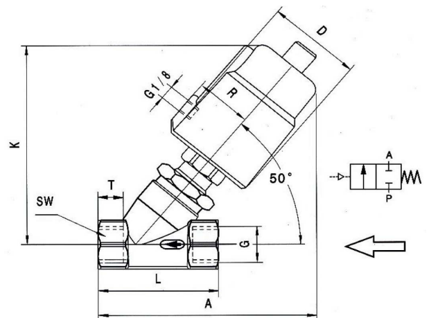
Spring return actuator, Normally closed (NC)
