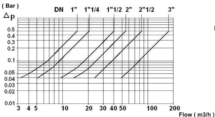
HEAD LOSS GRAPH :
