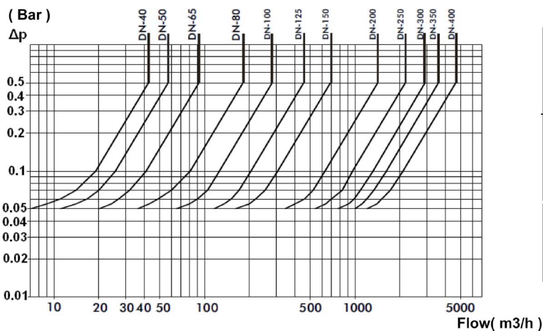
HEAD LOSS GRAPH:
